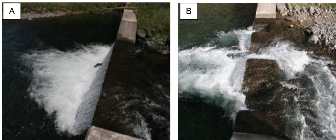
Fig. 8 Check dam before and after modification by making slits and notches
