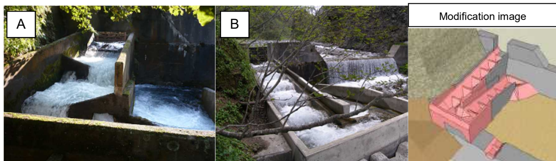
Fig. 2 Fishway at a check dam before and after modification
